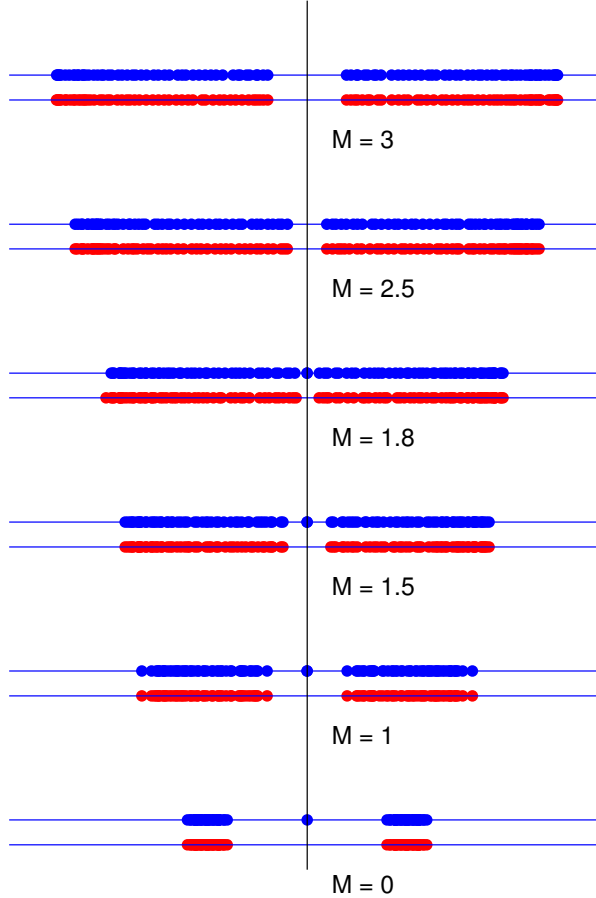
Figure 4: Spectral gaps
