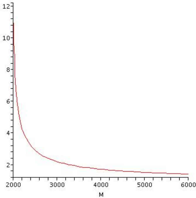
FIG. 10.3. Estimate for the “probabilistic” condition number \|\delta p\|/\|\delta y\| with a probability of at least 0.9
