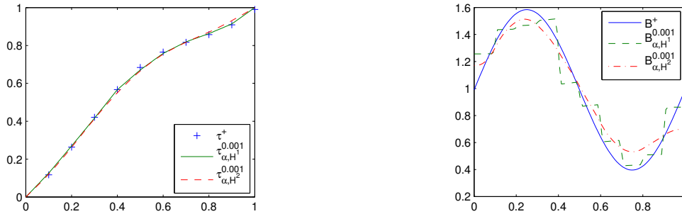
Figure 2: Left: The true maturities \tau^\delta and the regularized approximations \tau_\alpha^\delta for H^1 and H^2 regularization. Right: the underlying term structure B^\dagger and the corresponding reconstructions B_\alpha^\delta (cf. Table 2).
