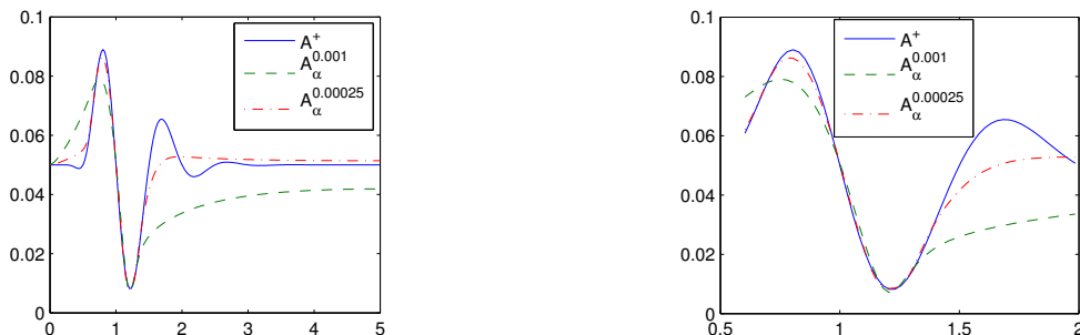
Figure 1: The true smile A^\dagger and the reconstructions A_\alpha^\delta for \delta = 0.001 and \delta = 0.00025 (cf. Table 1).
